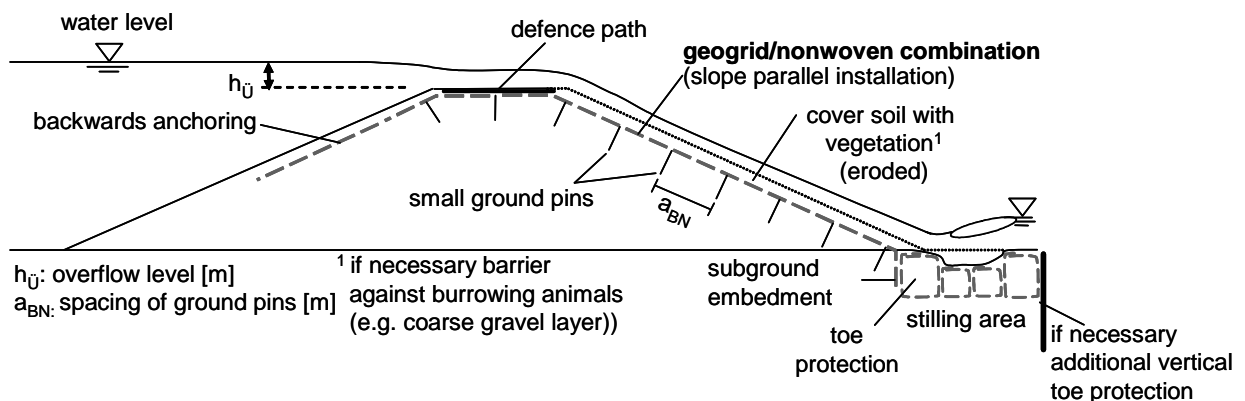
Fig. 9 Overflow protection per method (II), embankment parallel with geogrid/nonwoven combinations and ground pins (Haselsteiner et al. 2007)
