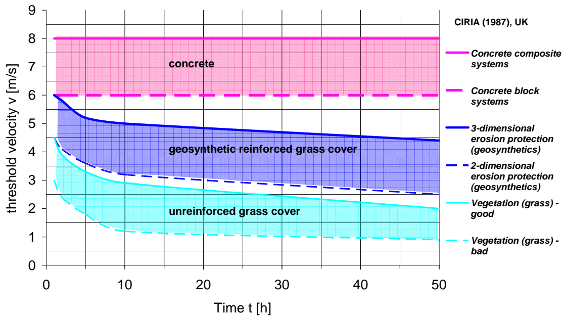
Fig. 8 Effectiveness of non-armored and armored grass covers on dam embankments during overflow (CIRIA 1987)
