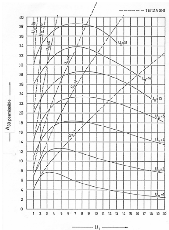
Fig. 6 Diagram by Ziem's for the dimensioning of granular filters compared to the filtration rules by Terzaghi (Teindl 1980)
