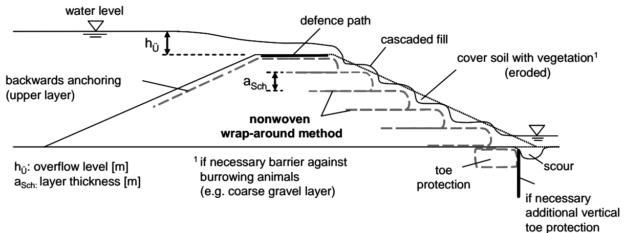
Fig. 10 Integrated overflow protection per method (III) in envelope method (Haselsteiner et al. 2007)
