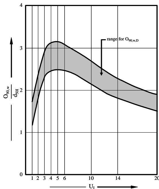
Fig. 7 Range of design values of O_{90,w,D} as function of d_{50I} and U_I of the base soil
