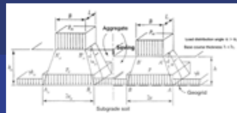
Fig 1. Load distribution angle with Combigrid®
